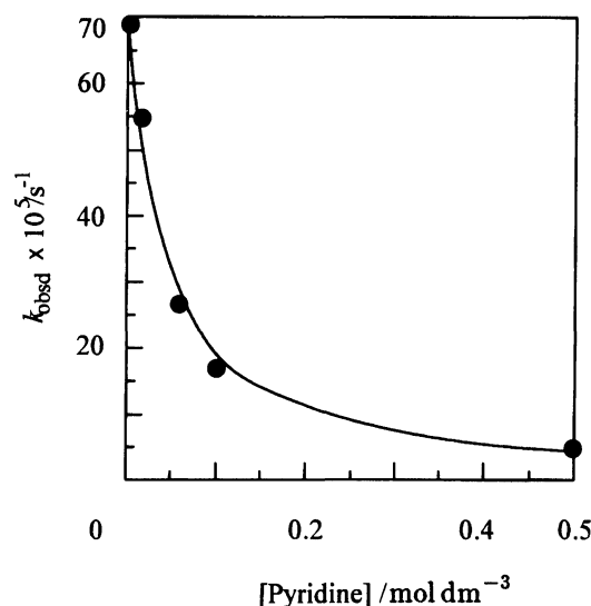
Fig. 2. Correlation between pyridine added and k_{\text{obsd}} in the reaction of complex 2 with methyl acrylate. [\mathbf{3}]_{t=0} = 0.03 \text{ mol dm}^{-3} . Solvent = \text{CH}_2\text{Cl}_2 : acetone (2 : 1). Temp = 5 °C.
