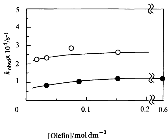
Fig. 1. Relation between concentration of added olefins and reaction rate. [\mathbf{3}]_{t=0} = 0.03 \text{ mol dm}^{-3} . Solvent = \text{CH}_2\text{Cl}_2 : acetone (2 : 1). Temp = 5 °C. ○ = Methyl acrylate, ● = Styrene.
